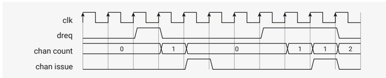
Figure 13. DREQ counting
