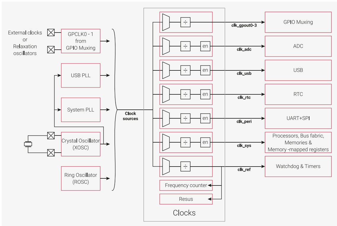
Figure 28. Clocks overview
