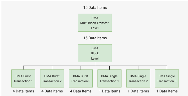
Figure 165. Breakdown of DMA Transfer into Single and Burst Transactions. Block size, DMA.CTLx.BLOCK_TS = 15 . Number of data items per burst transaction, DMA.CTLx.DEST_MSIZ = 4 . SSI transmit FIFO watermark level, SSI.DMATDLR = DMA.CTLx.DEST_MSIZ = 4
