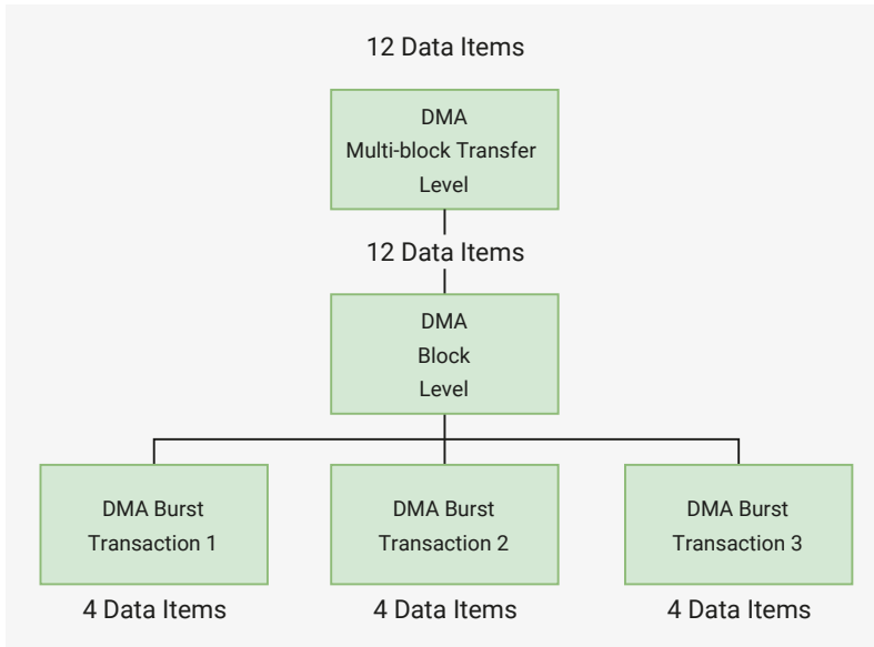
Figure 164. Breakdown of DMA Transfer into Burst Transactions. Block size, DMA.CTLx.BLOCKS_TS = 12 . Number of data items per source burst transaction, DMA.CTLx.SRC_MSIZ = 4 . SSI receive FIFO watermark level, SSI.DMATDLR + 1 = DMA.CTLx.SRC_MSIZ = 4
